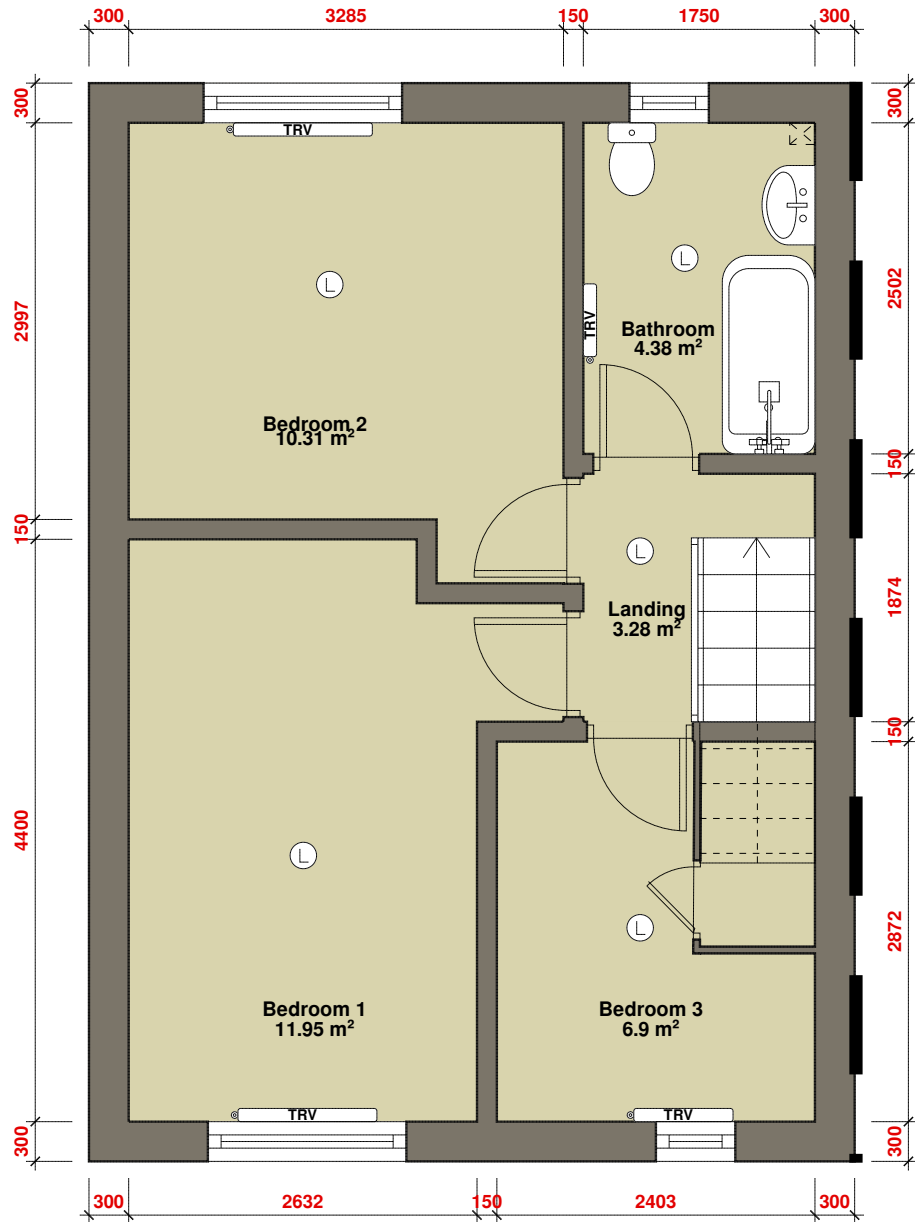
1st Floor - Surveyors Ltd - Example CAD Floor Plan
