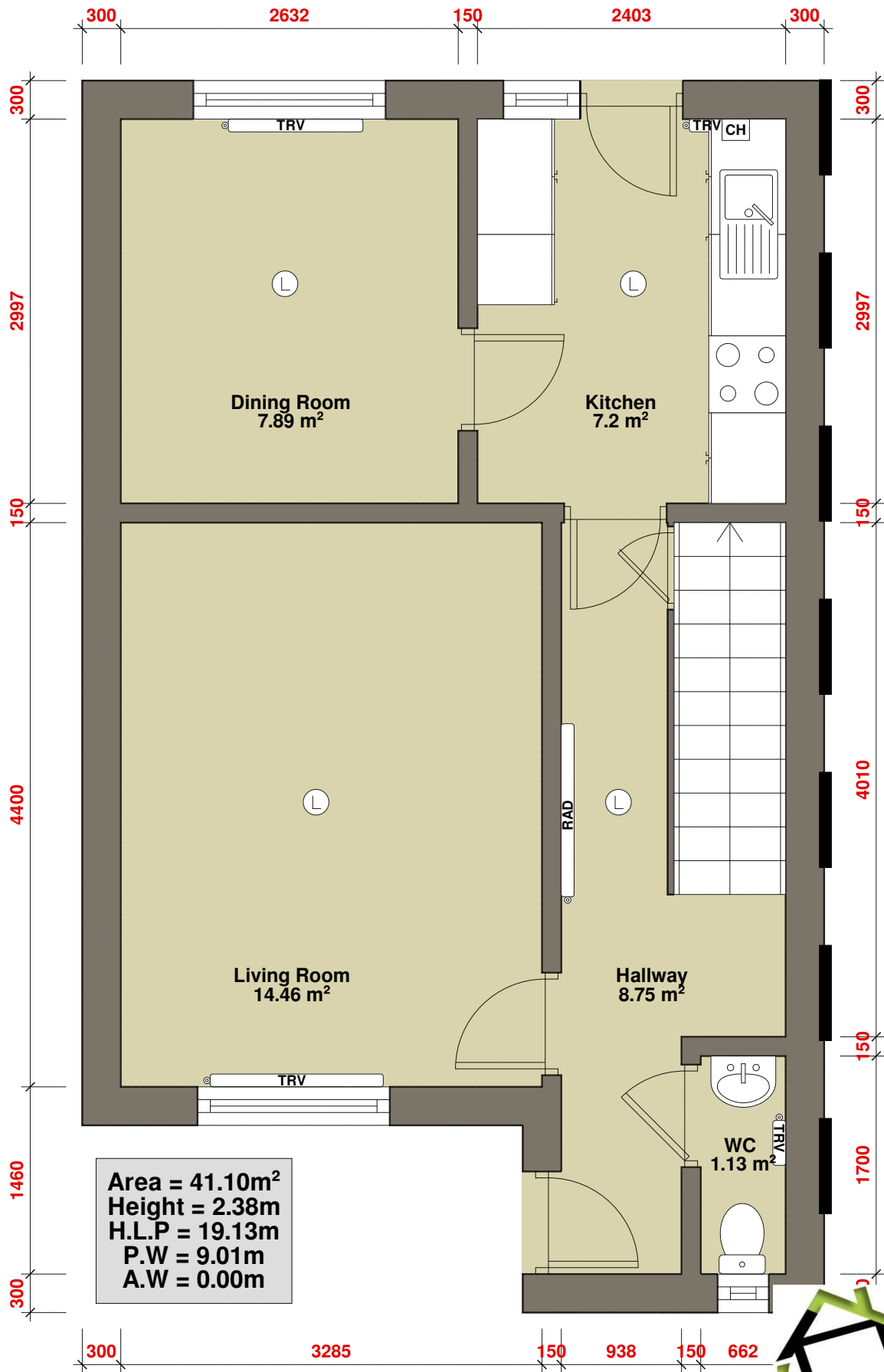
Ground Floor - Surveyours Ltd - Example CAD Floor Plan
